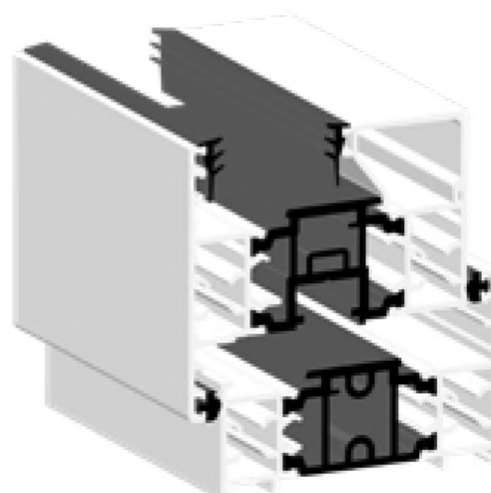
Contemporary sash, Standard frame
