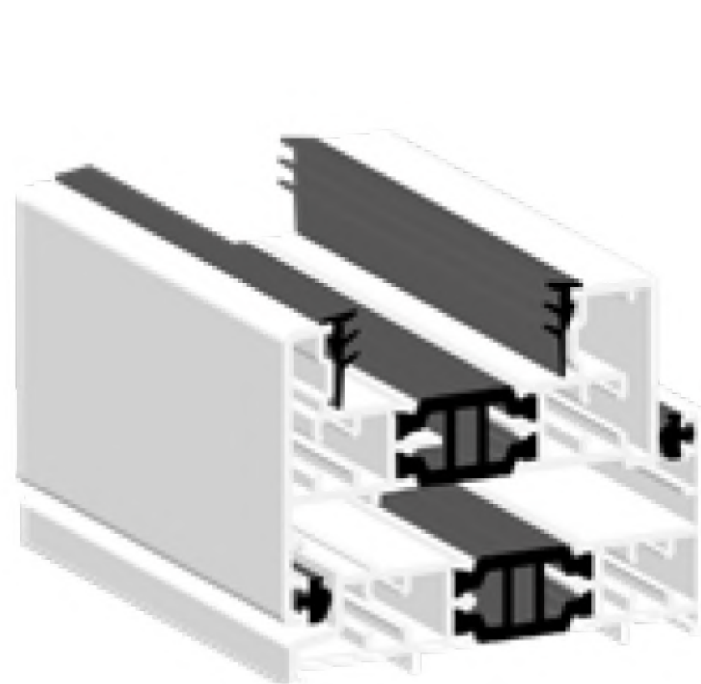
Contemporary sash, Flush frame
