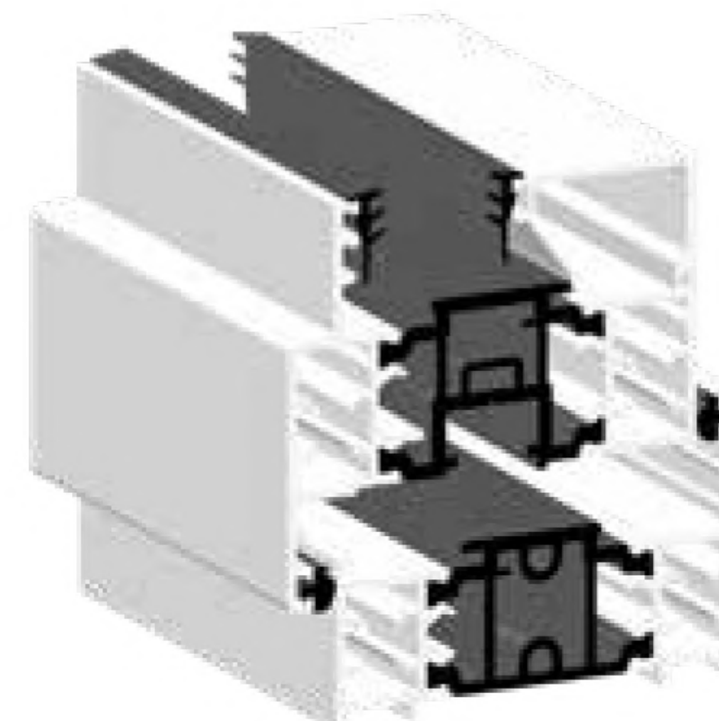
Stepped sash, Standard frame
